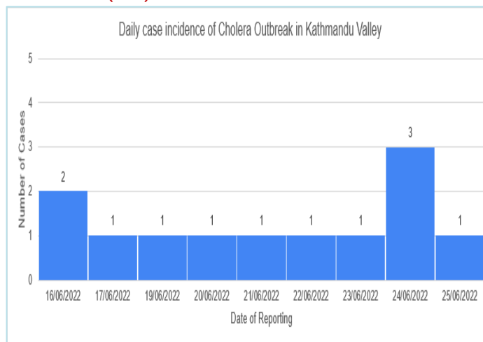
Epidemic curve of reported cases of Cholera in Kathmandu Valley, as of 26 th June 2022 (n=12)
