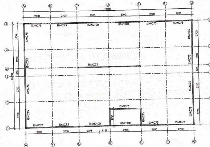
EAVES LEVEL TIE BEAM LAYOUT PLAN
