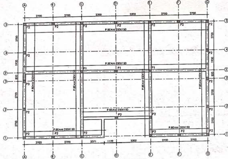
PLINTH BEAM /POST LAYOUT PLAN
