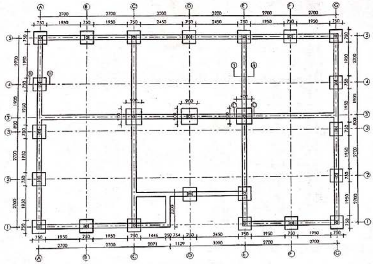
FOUNDATION LAYOUT PLAN
