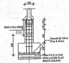
POST/COLUMN CONNECTION DETAILS SCALE 1:25
