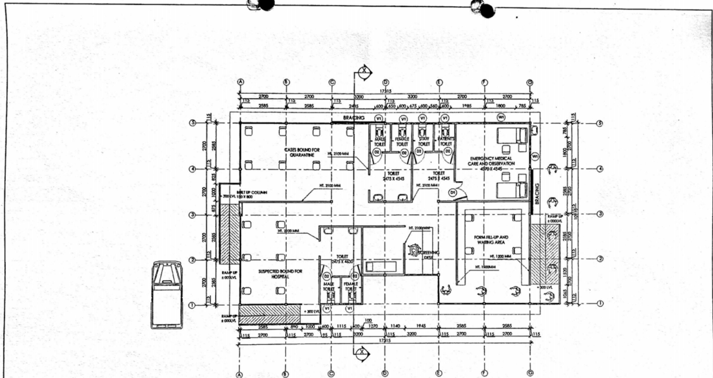
GROUND FLOOR PLAN Area : 180 SQ. M. (excluding Ramp)
