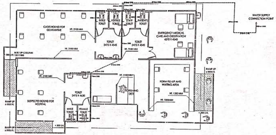
WATER SUPPLY LAYOUT PLAN
