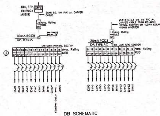
DB SCHEMATIC
