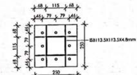
8 NOS. 120 BOLTS 450mm DEEP 10mm THICK BASE PLATE BASE PLATE PLAN (P1)
